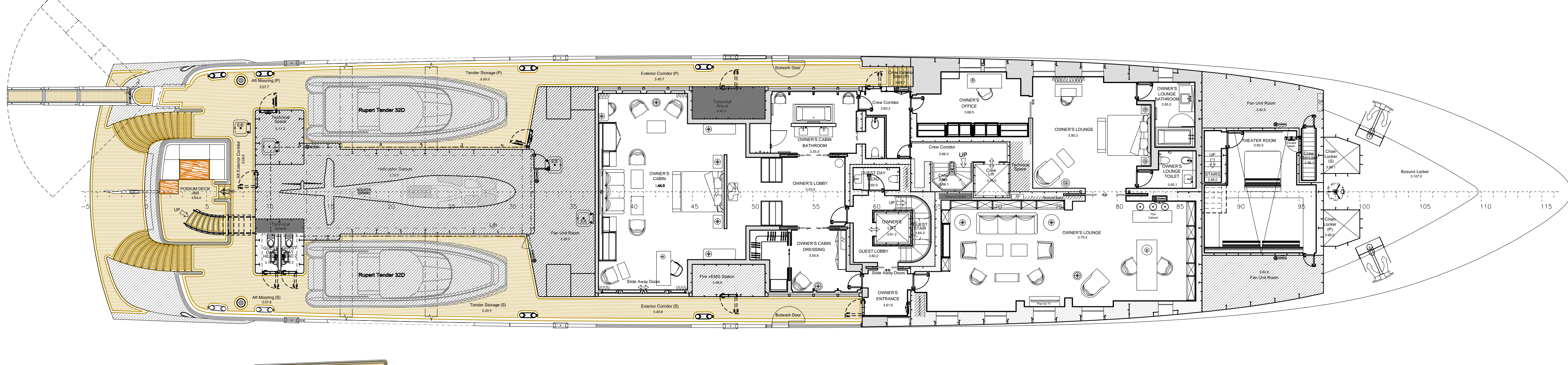
MAIN DECK at 7000 from B.L.
