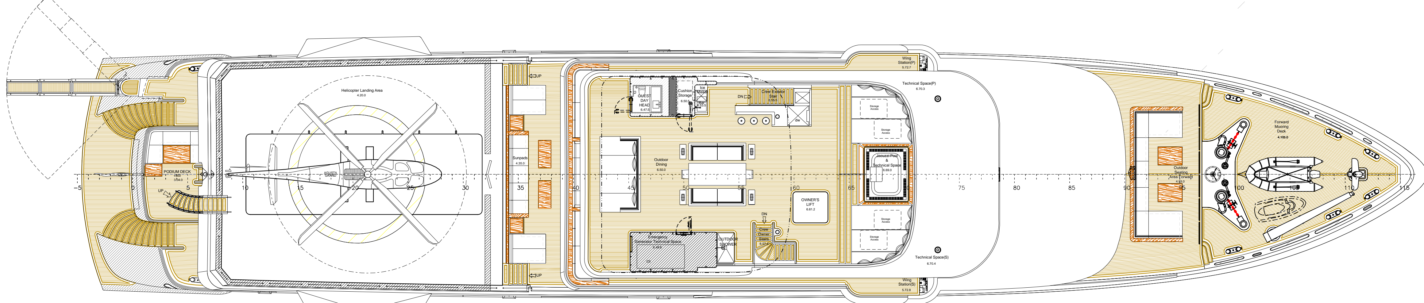
SUN DECK at 15200 from B.L.
